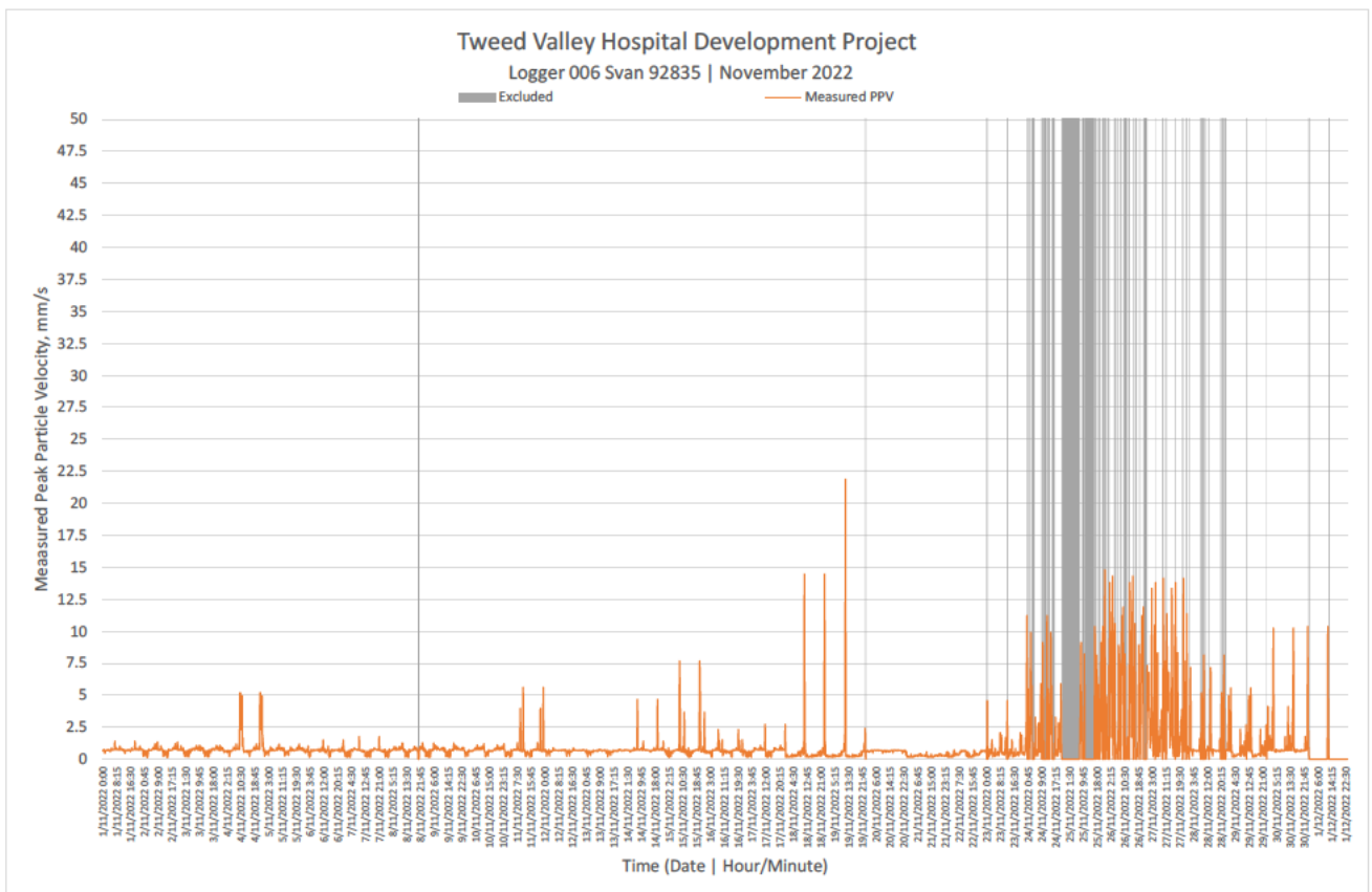
Figure 5 Velocity over time (Logger 006 – Residential/Commercial)
