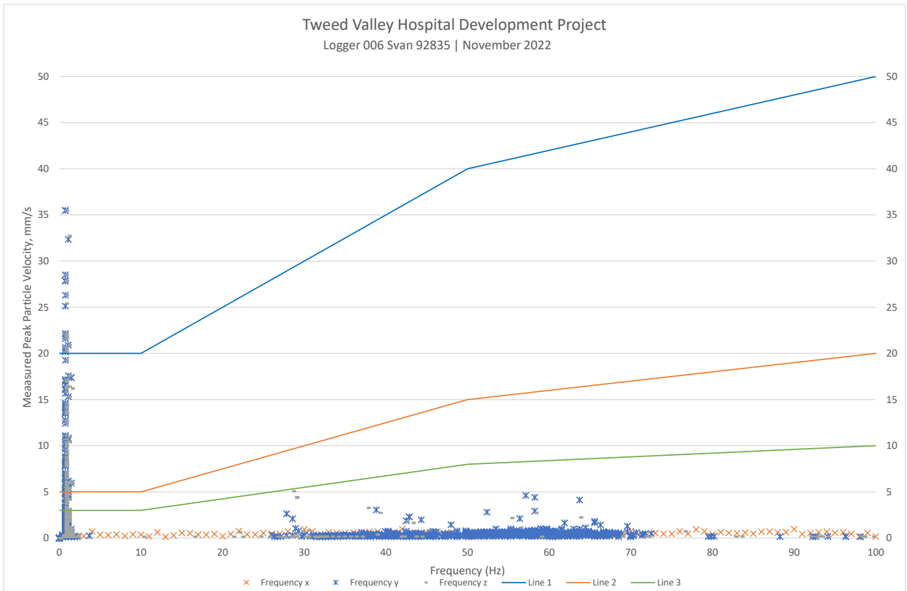
Figure 6 Velocity over frequency (Logger 006)
