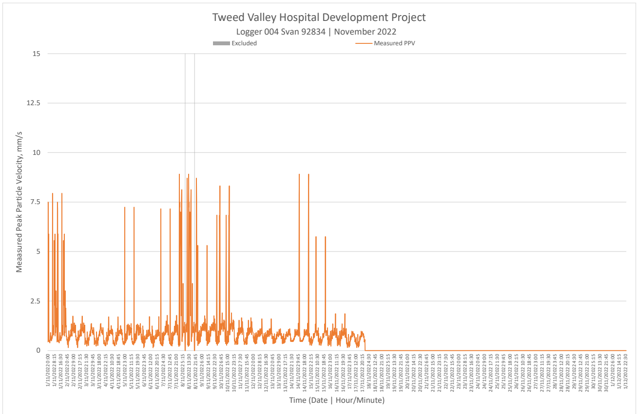
Figure 2 Velocity over time (Logger 004)
