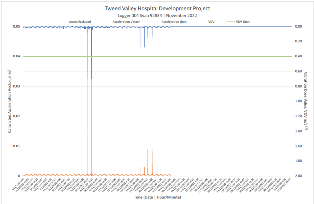
Figure 8 Acceleration and Vibration Dose Value over time (Logger 004)
