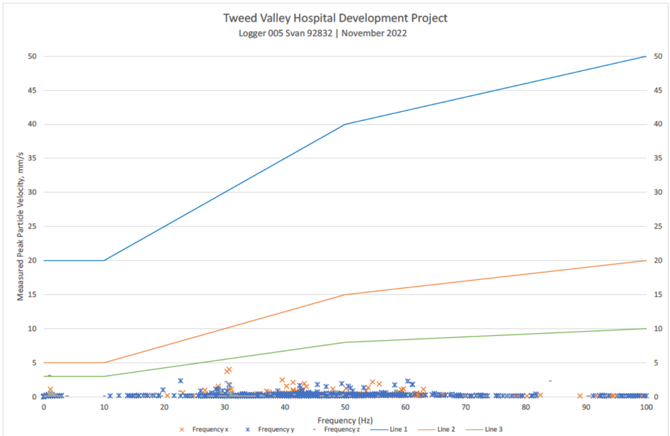
Figure 4 Velocity over frequency (Logger 005)
