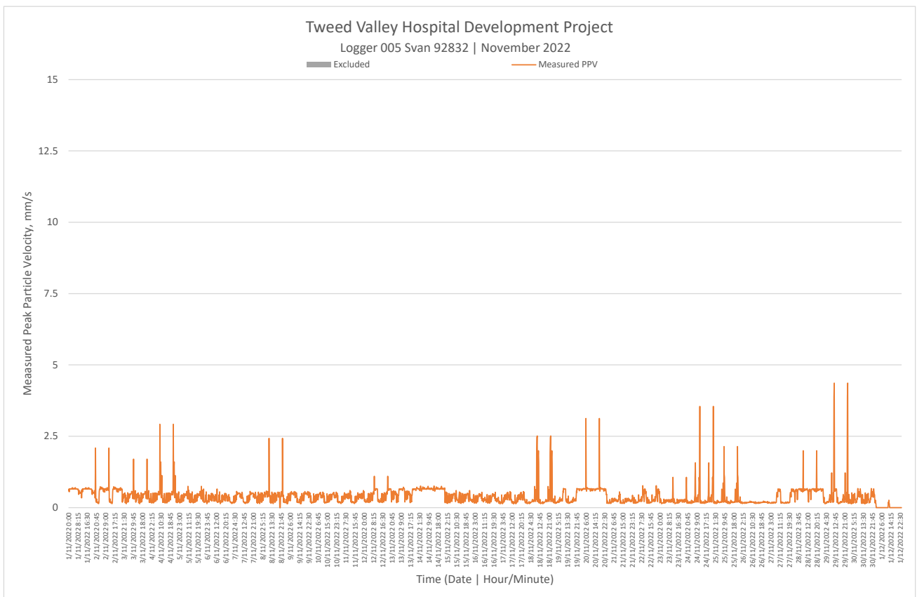
Figure 3 Velocity over time (Logger 005)
