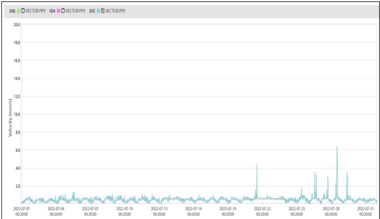
Figure 2. Vibration data at location 005 | TAFE West | July 2022
