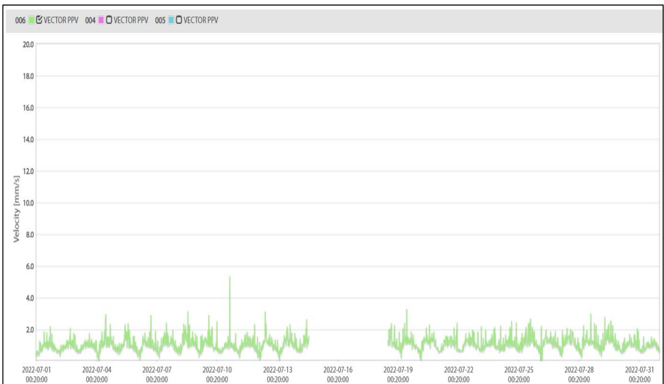
Figure 3. Vibration data at location 006 | Mate and Matt's | July 2022
