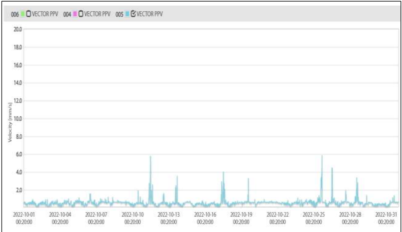
Figure 2. Vibration data at location 005 | TAFE West | October 2022
