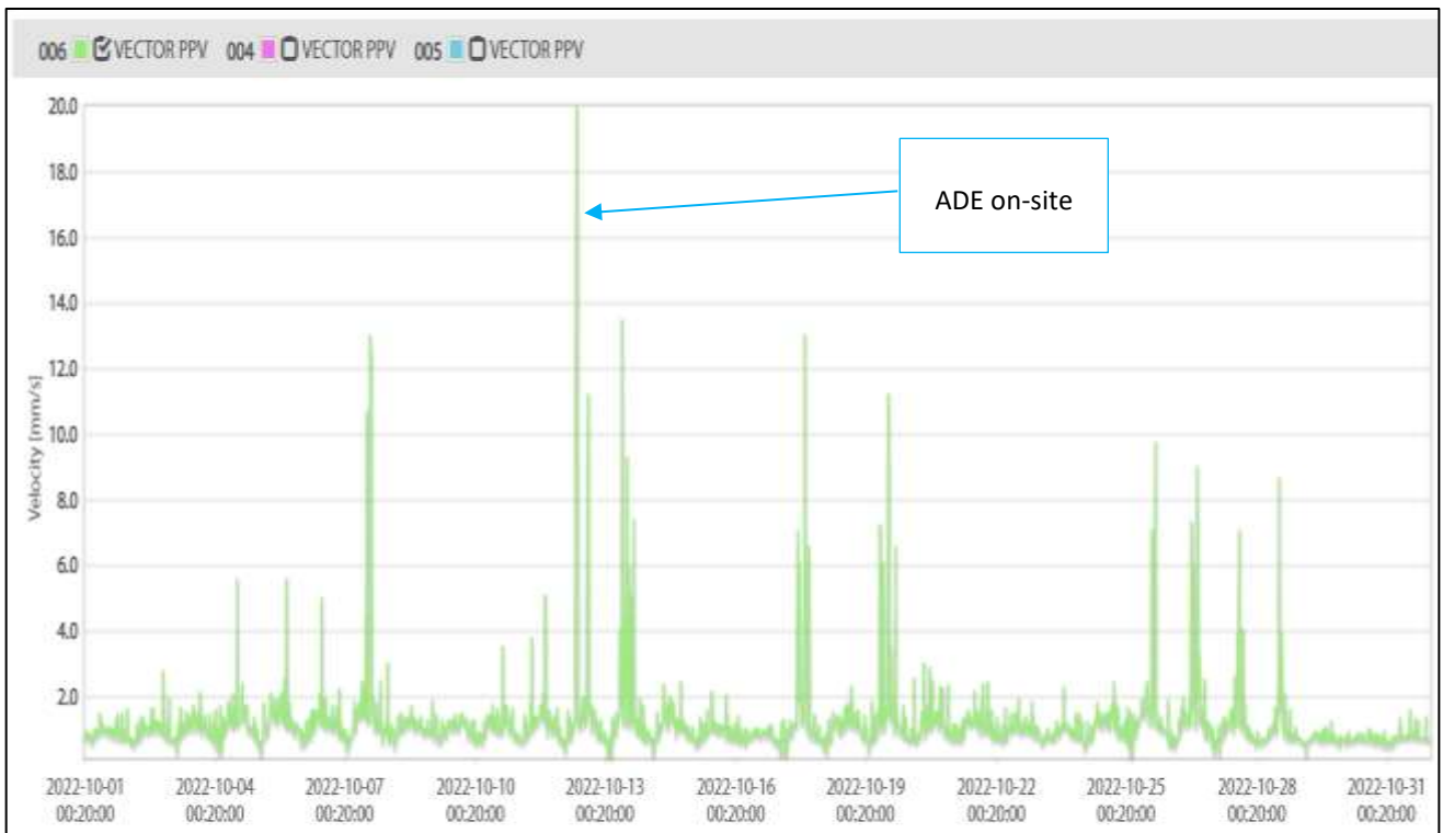
Figure 3. Vibration data at location 006 | Mate and Matt's | October 2022
