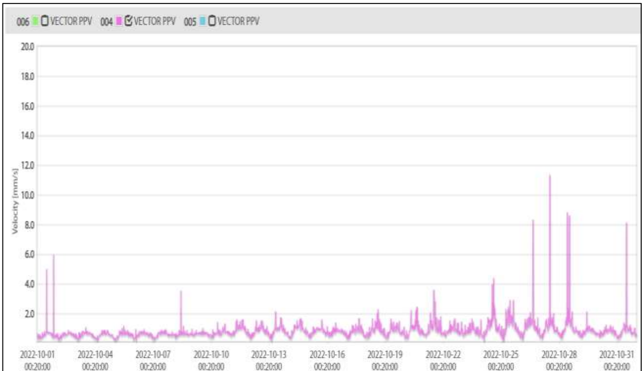
Figure 1. Vibration data at location 004 | TAFE East | October 2022
