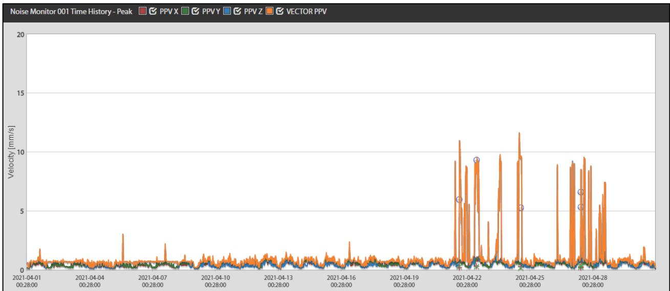
Figure 1 Vibration data at location 001 | Adjacent carpark | April 2021
