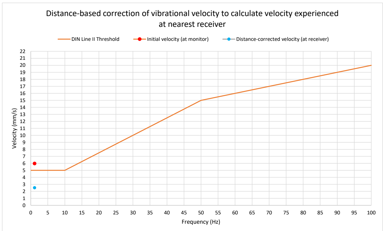
Figure 4 Distance corrected PPV values (monitoring location 001)
