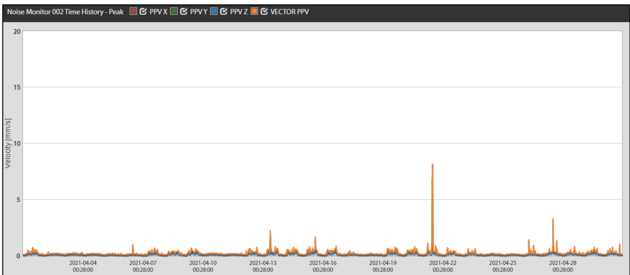
Figure 2 Vibration data at location 002 | Central monitor | April 2021
