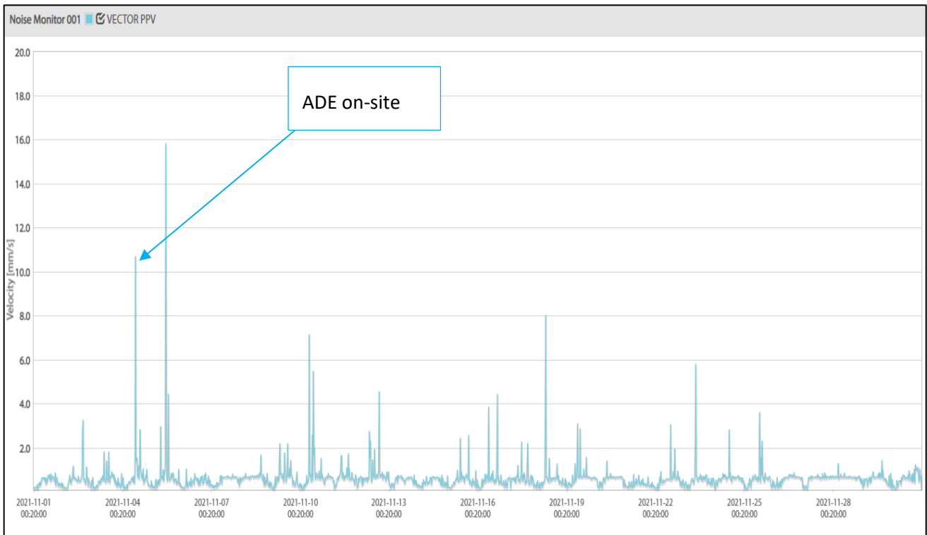
Figure 1. Vibration data at location 001 | Adjacent carpark | November 2021.
