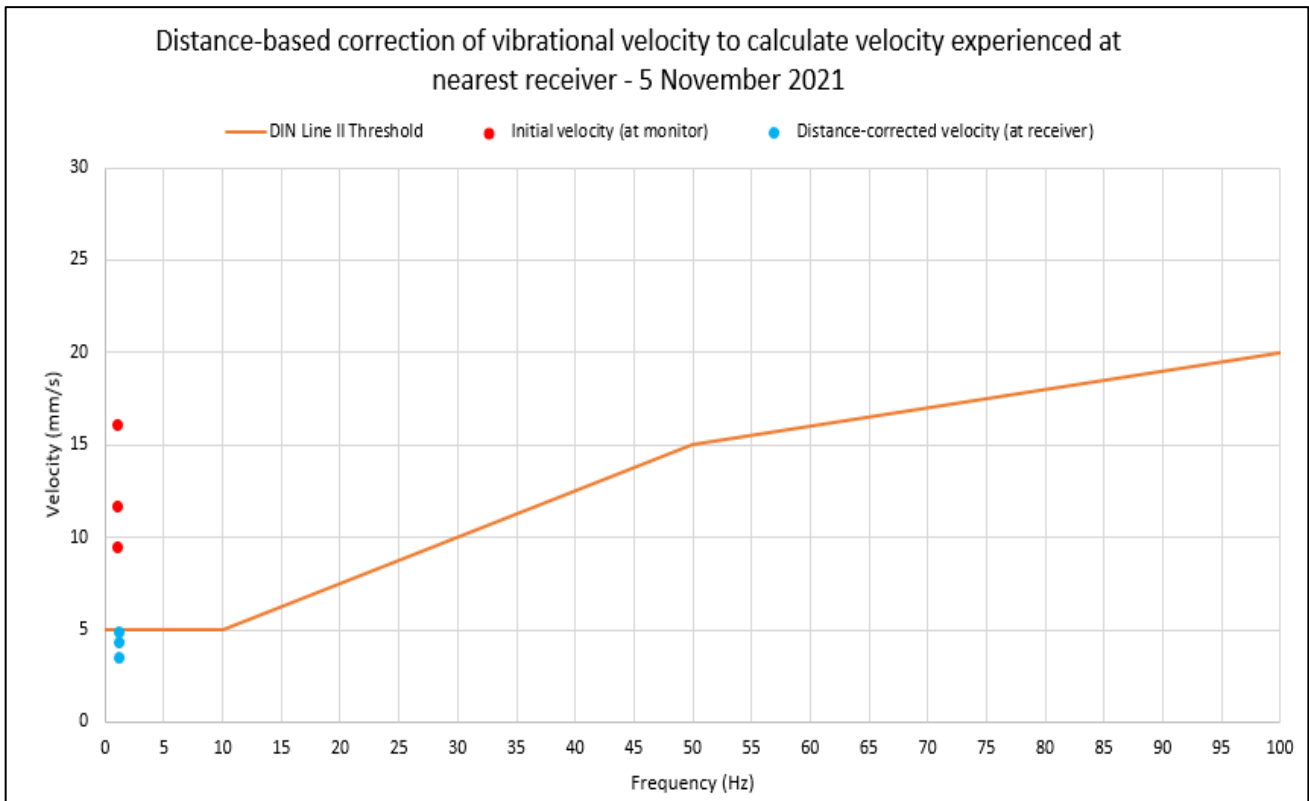
Figure 4 Distance corrected PPV values (monitoring location 001)
