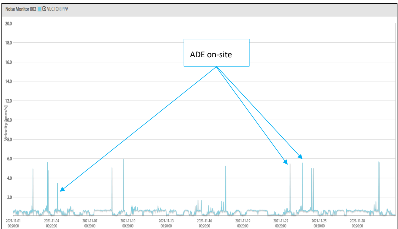
Figure 2. Vibration data at location 002 | Central monitor | November 2021
