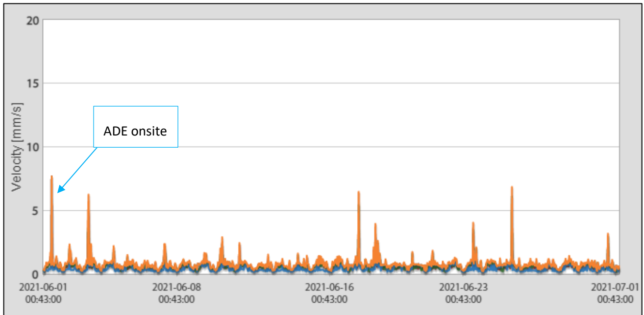
Figure 1 Vibration data at location 001 | Adjacent carpark | June 2021
