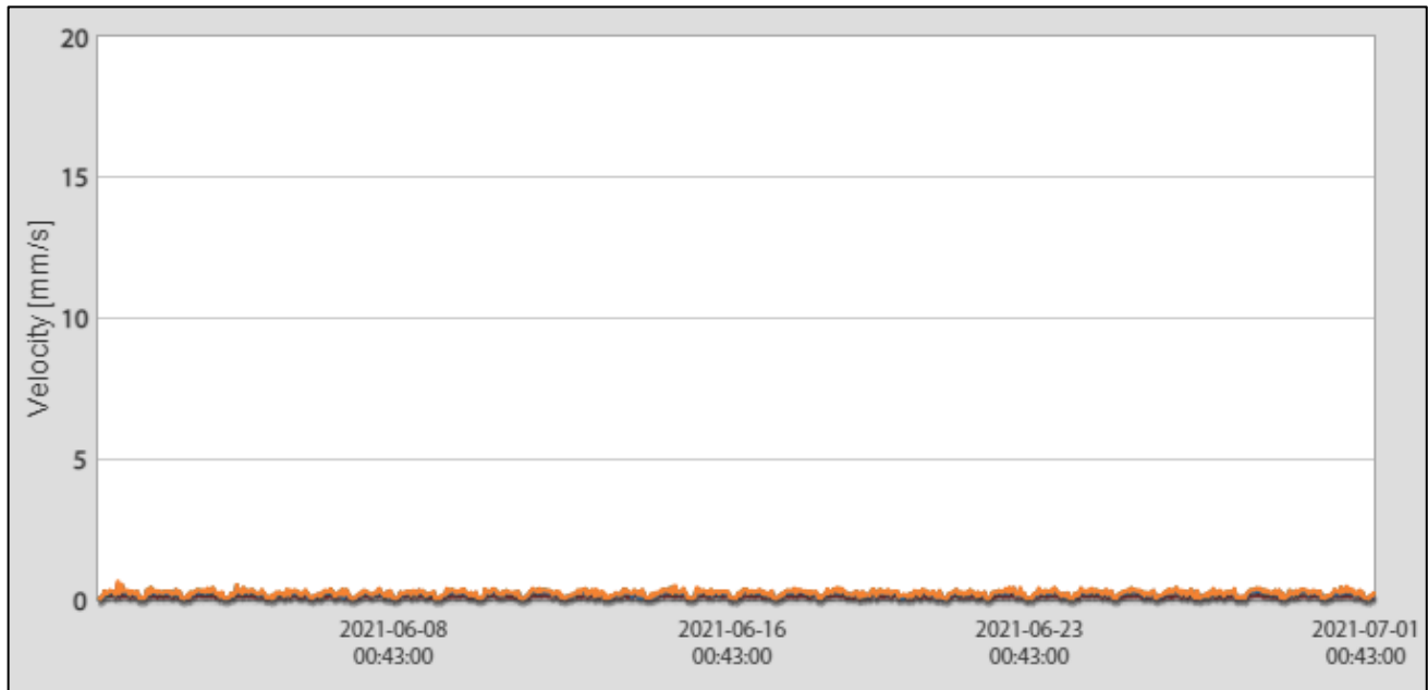
Figure 3 Vibration data at location 003 | Eastern section | June 2021
