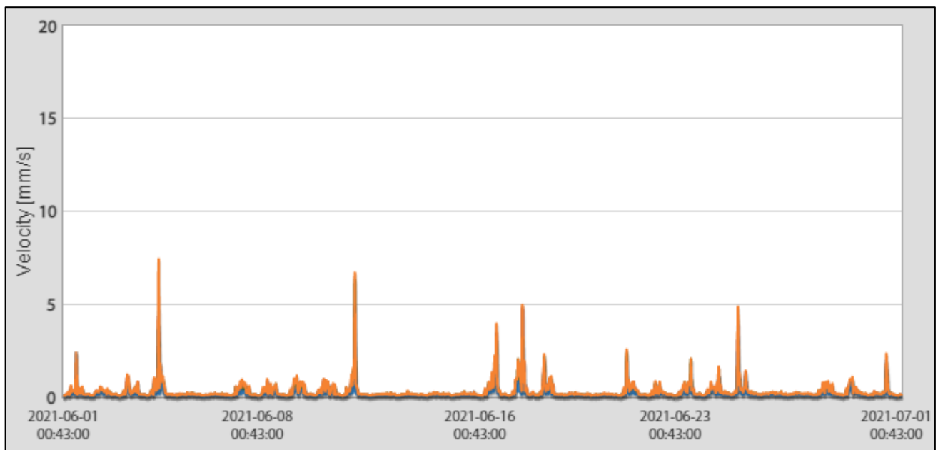
Figure 2 Vibration data at location 002 | Central monitor | June 2021
