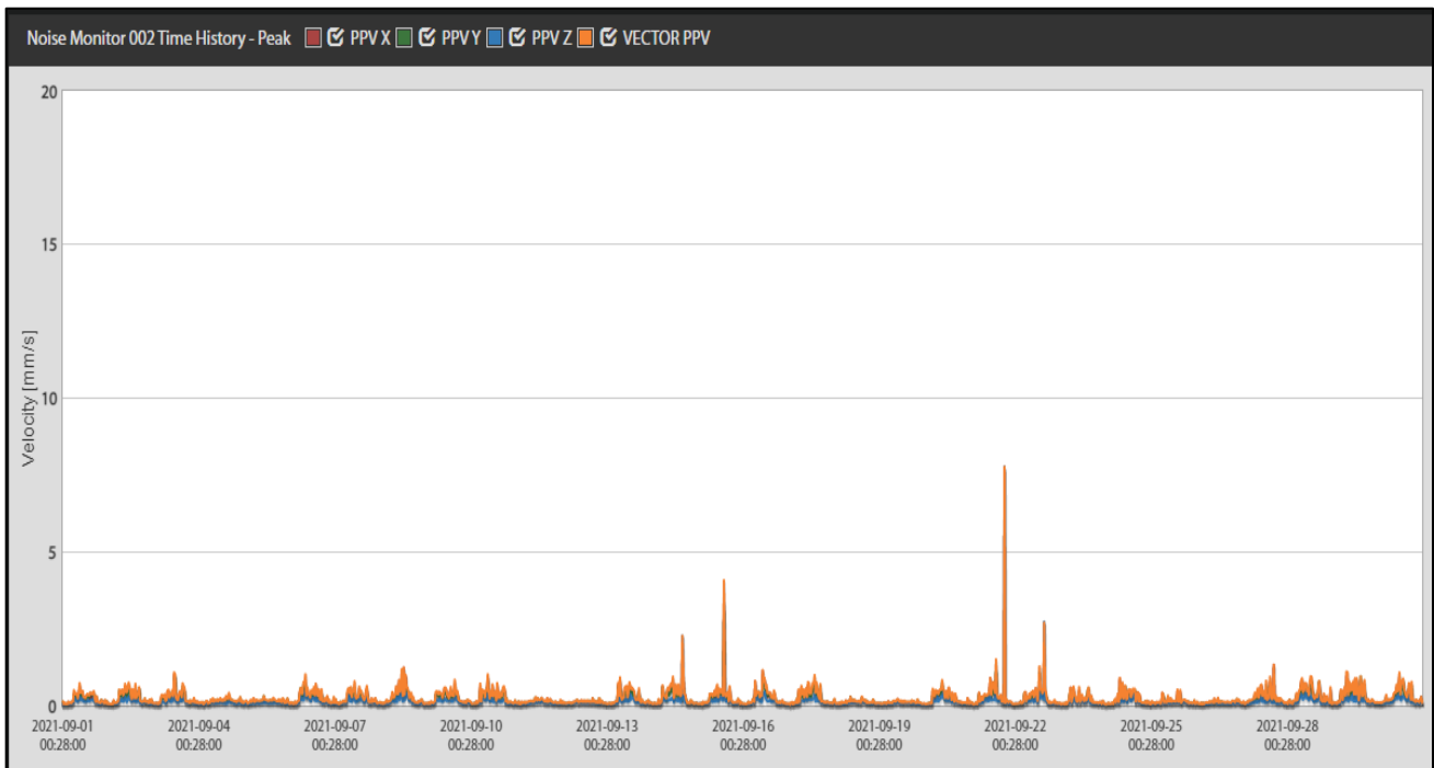
Figure 2. Vibration data at location 002 | Central monitor | September 2021
