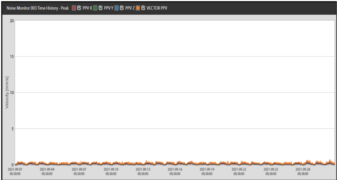
Figure 3. Vibration data at location 003 | Eastern section | September 2021
