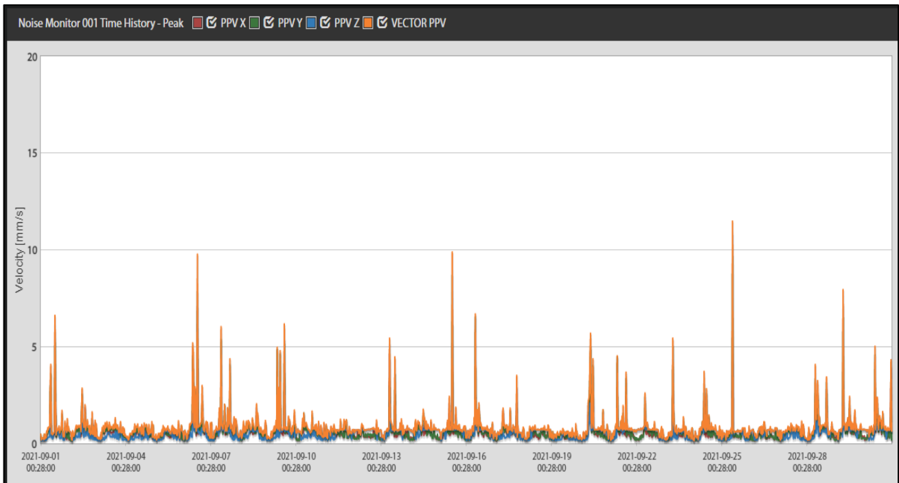
Figure 1. Vibration data at location 001 | Adjacent carpark | September 2021.
