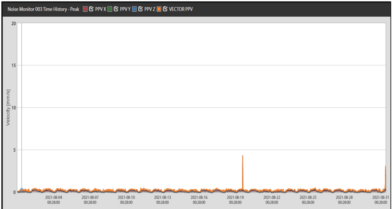
Figure 3. Vibration data at location 003 | Eastern section | August 2021.
