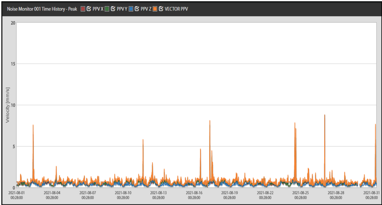
Figure 1. Vibration data at location 001 | Adjacent carpark | August 2021.
