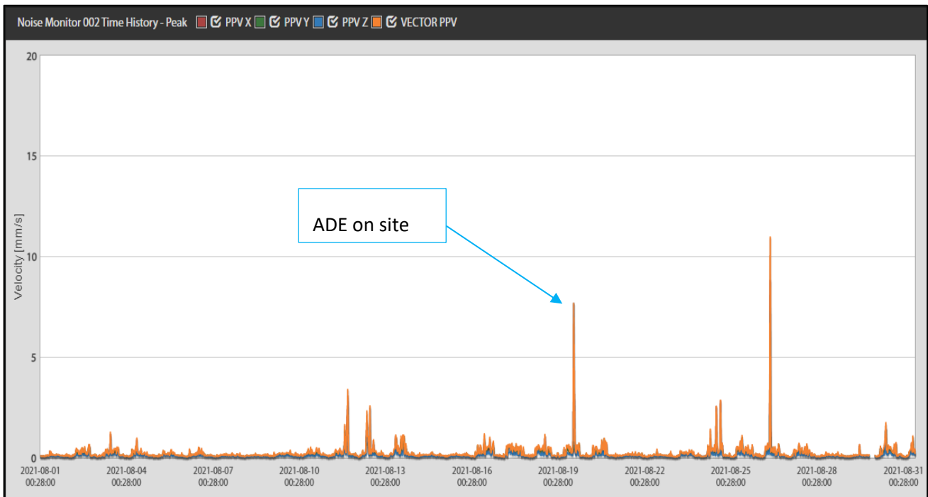
Figure 2. Vibration data at location 002 | Central monitor | August 2021.
