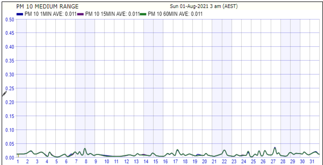
Figure 2. Summary of PM10 from the real time monitoring at location 002 – Central location for the month of August 2021.
