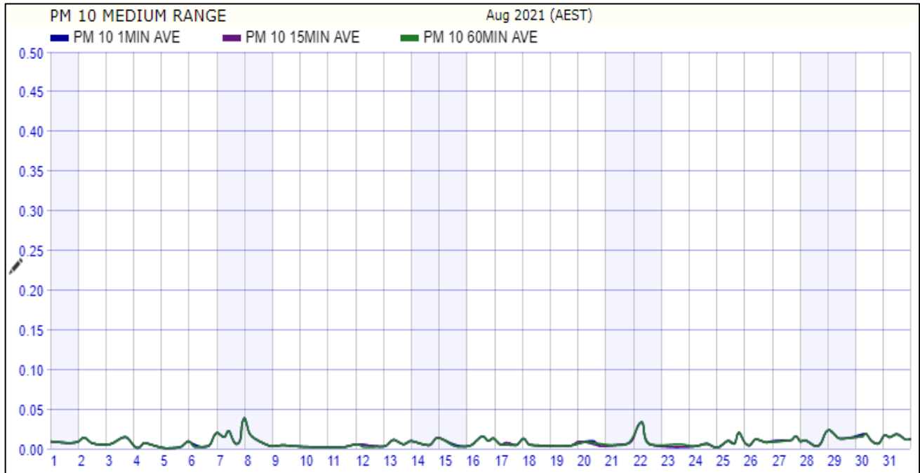
Figure 1. Summary of PM10 from the real time monitoring at location 001 – Adjacent to the carpark for the month of August 2021.
