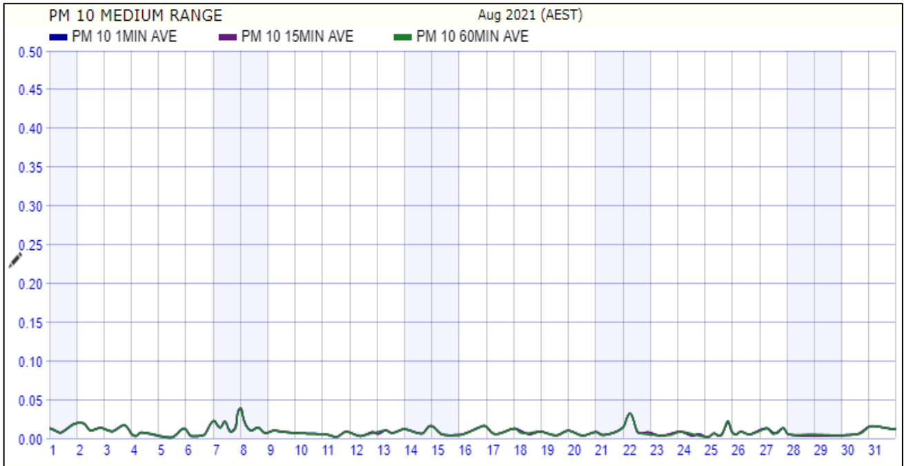
Figure 3. Summary of PM10 from the real time monitoring at location 003 – Eastern Section of site for the month of August 2021.
