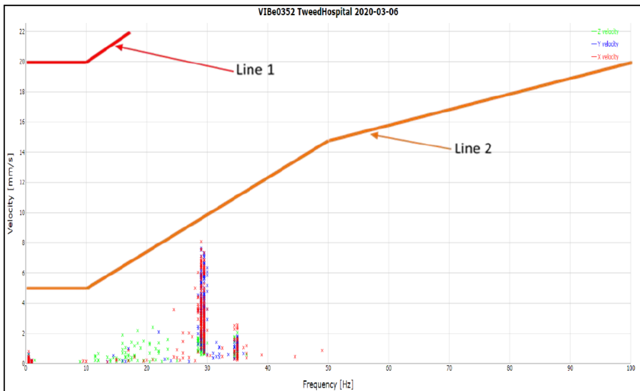
Figure 8. Results of the exceedance on Friday 6 th March 2020 at monitoring location 001 – adjacent carpark monitor.
