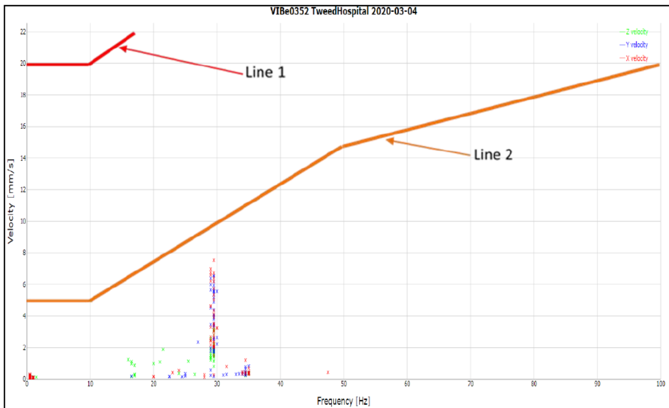
Figure 6. Results of the exceedance on Wednesday 4 th March 2020 at monitoring location 001 – adjacent carpark monitor.
