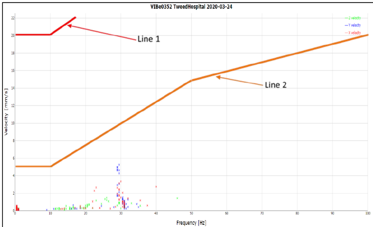
Figure 12. Results of the exceedance on Friday 24 th March at monitoring location 001 – adjacent carpark monitor.
