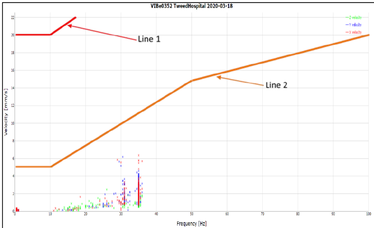
Figure 11. Results of the exceedance on Wednesday 18 th March at monitoring location 001 – adjacent carpark monitor.
