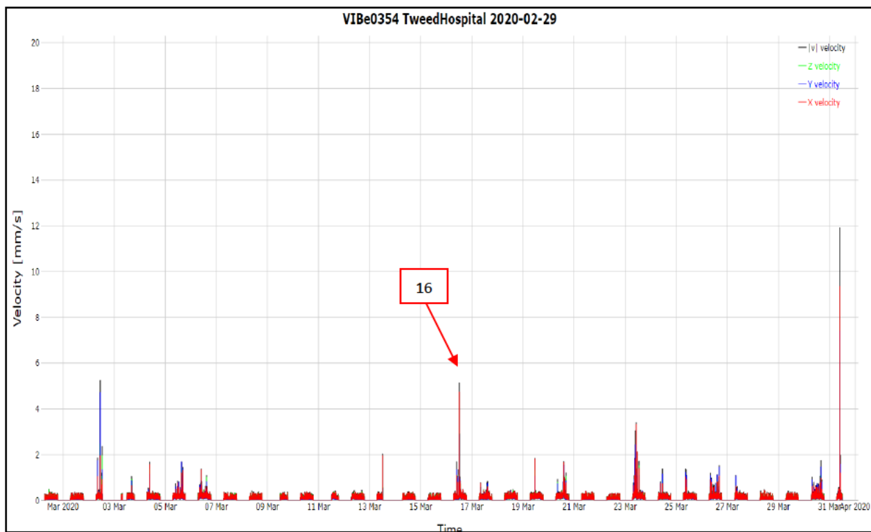
Figure 4. Results of the vibration monitoring from Sunday 1 st March 2020 to Tuesday 31 st March 2020 at monitoring location 003 – Eastern section of site.
