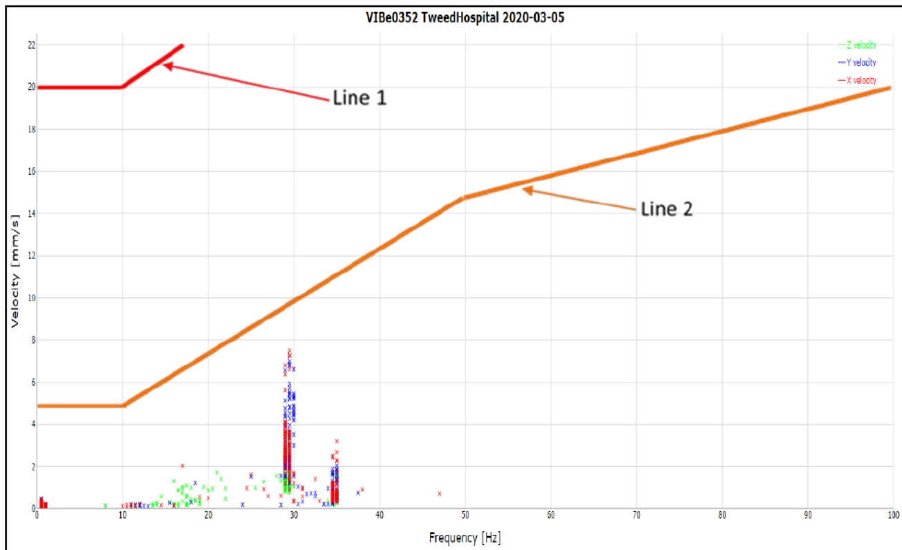
Figure 7. Results of the exceedance on Thursday 5 th March 2020 at monitoring location 001 – adjacent carpark monitor.
