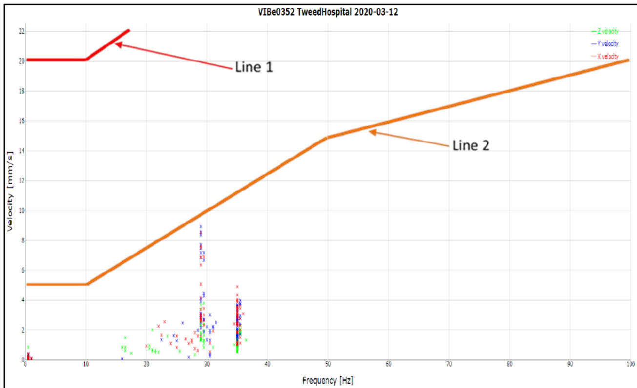
Figure 9. Results of the exceedance on Thursday 12 th March 2020 at monitoring location 001 – adjacent carpark monitor.
