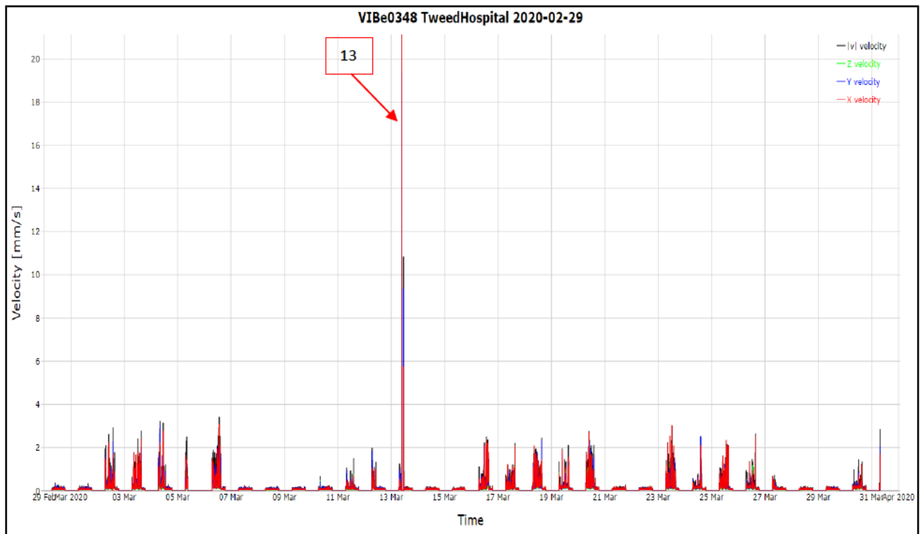
Figure 3. Results of the vibration monitoring from Sunday 1 st March 2020 to Tuesday 31 st March 2020 at monitoring location 002 – Central monitor.
