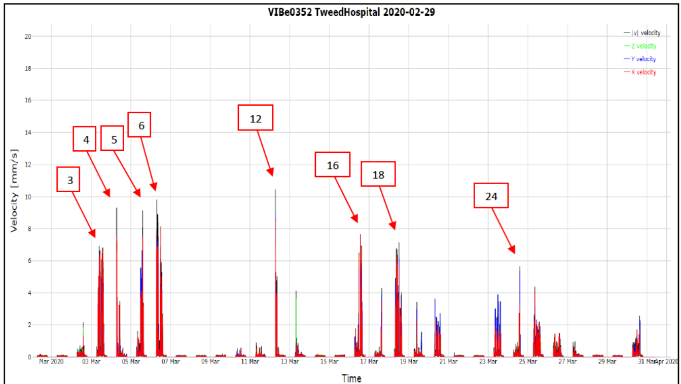
Figure 2. Results of the vibration monitoring from Sunday 1 st March 2020 to Tuesday 31 st March 2020 at monitoring location 001 – Adjacent carpark.
