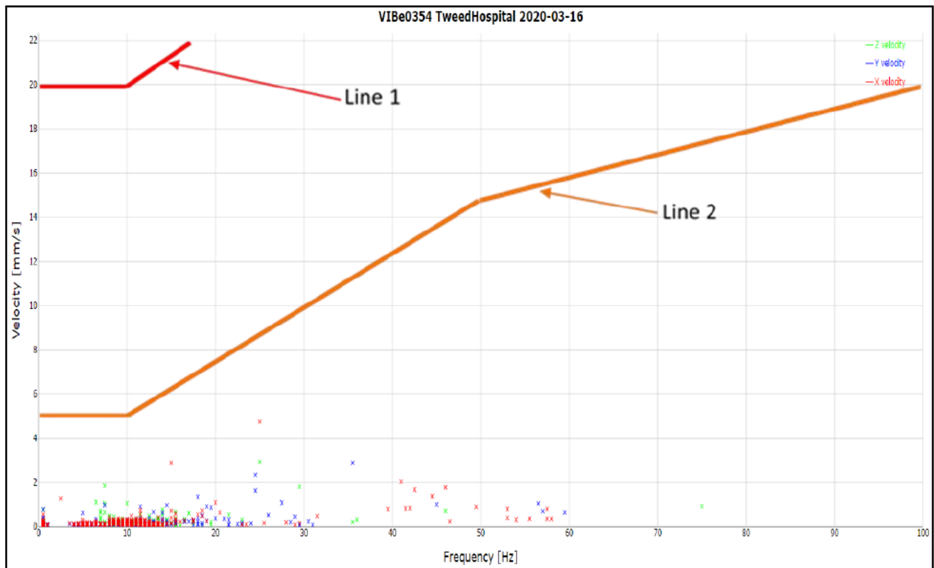
Figure 13. Results of the exceedance on Monday 16 th March at monitoring location 003 –Eastern Section of Site.
