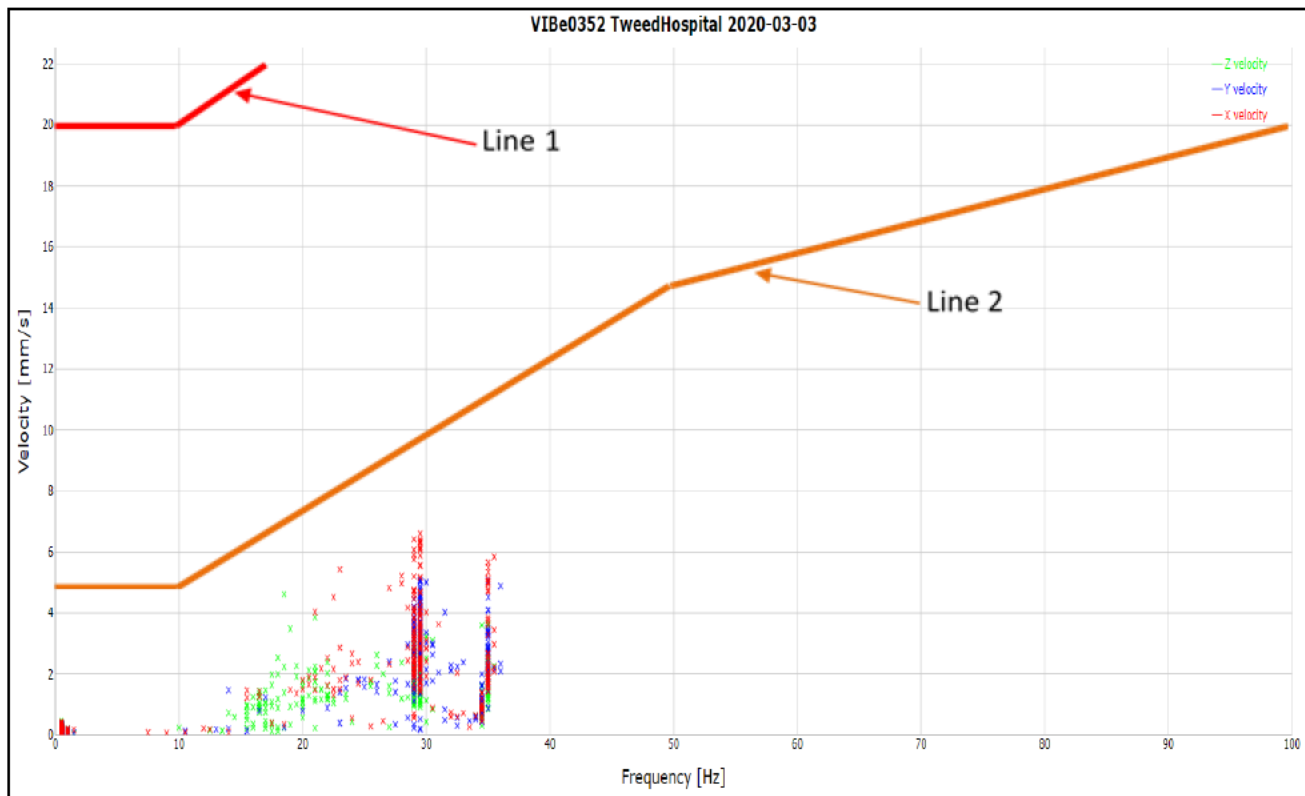
Figure 5. Results of the exceedance on Tuesday 3 rd March 2020 at monitoring location 001 – adjacent carpark monitor.
