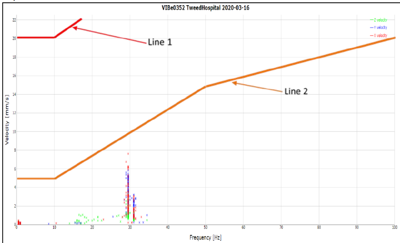
Figure 10. Results of the exceedance on Monday 16 th March at monitoring location 001 – adjacent carpark monitor.
